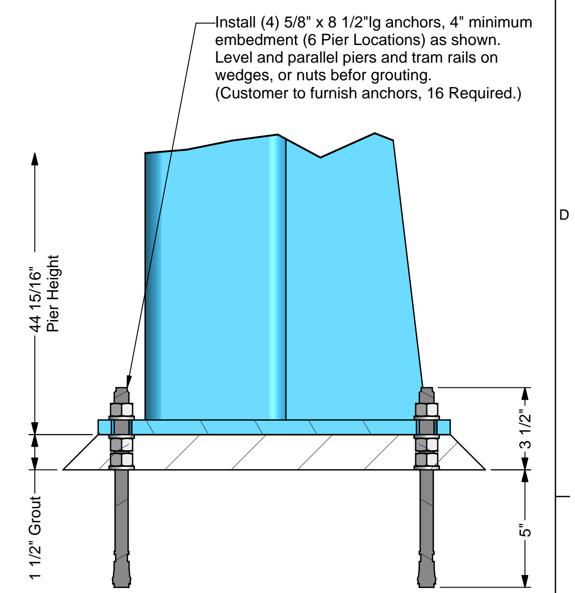
DETAIL A SCALE 1/4
